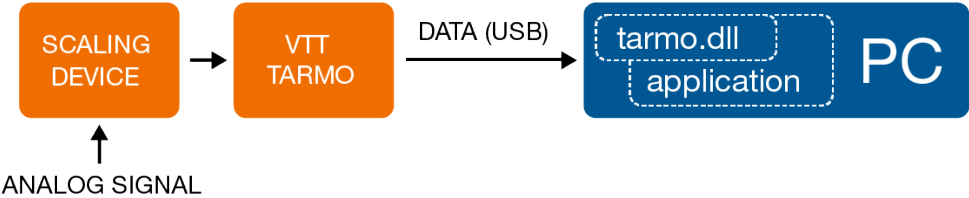
VTT Tarmo used as a sampling AC measurement standard. A separate scaling device can be used for extending the input range.
